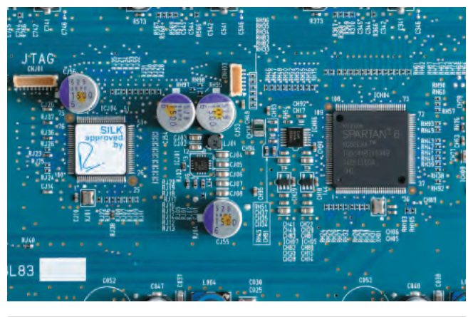
Silk processor on the analogue input board; the Silk DSP simulates the behaviour of the analogue pre-amp with transformer developed by Rupert Neve
