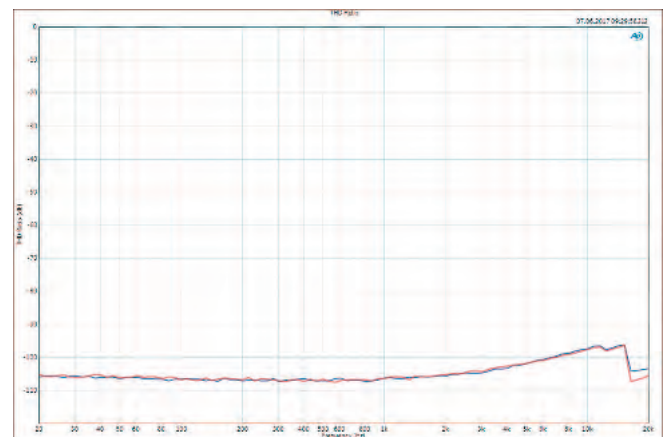
THD of pre-amp and ADC at 1 kHz and 0 dB gain depending on the frequency at -6 dBfs modulation corresponding to +18 dBu analogue input level (Fig. 3)
