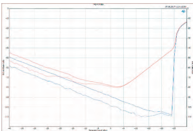
THD and THD+N from pre-amp and ADC at 1 kHz with (red) and without (blue) Silk depending on input level. The respective solid line shows the THD+N values; the dashed curve shows THD only (Fig. 16)
