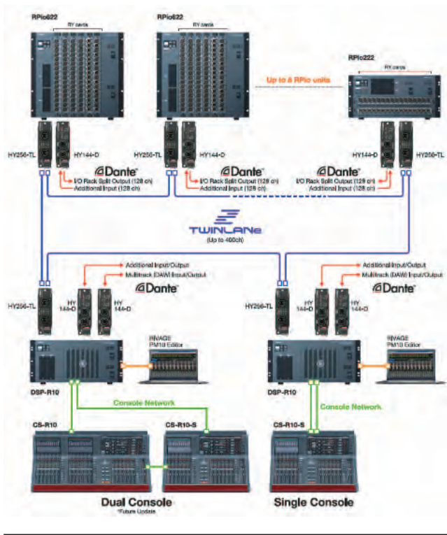
PM10 Rivage system in a large sample configuration with three consoles, two DSP units and three I/O racks. The core system is networked via a Yamaha TWINLANE ring. Connections to external devices with audio signals are made via Dante network. The consoles are connected to the DSP engines via the console network, also as a ring. (Fig. 1)
