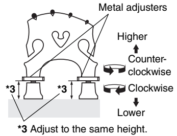
[Fig. 3: Adjusting bridge height]
